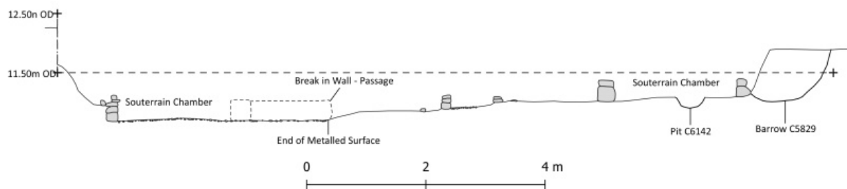
Profile through souterrain
