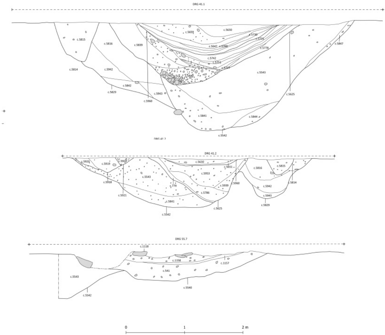
Sections of C5542
