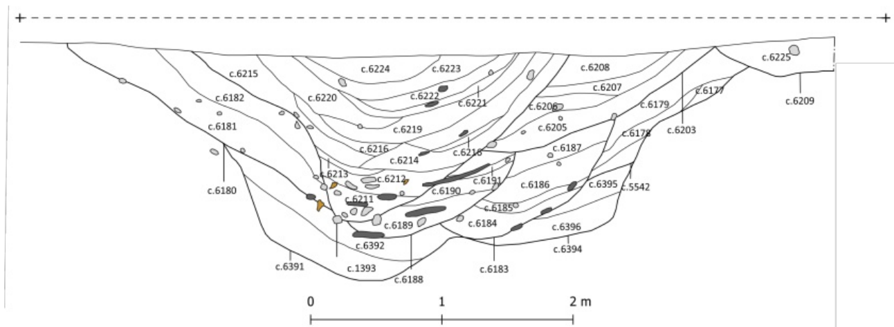
Section of entrance into western cemetery
