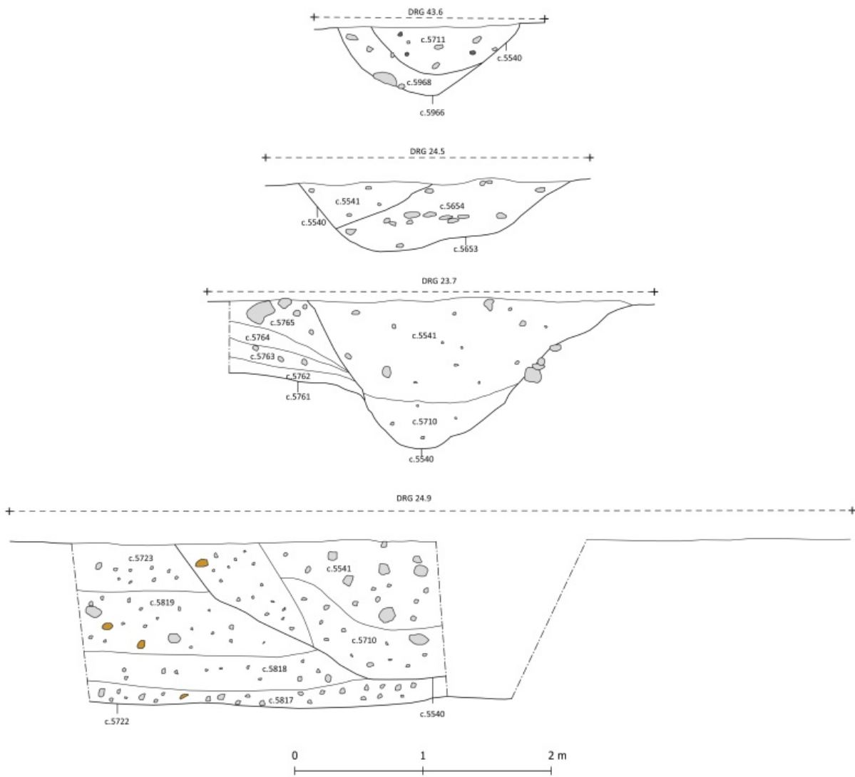
Sections of C5540
