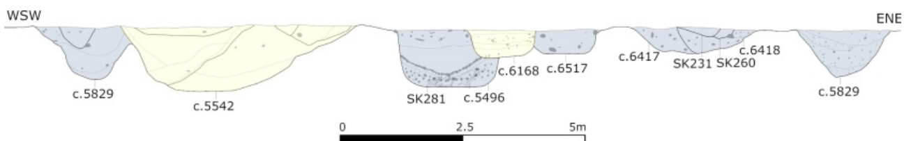
Section through ring ditch
