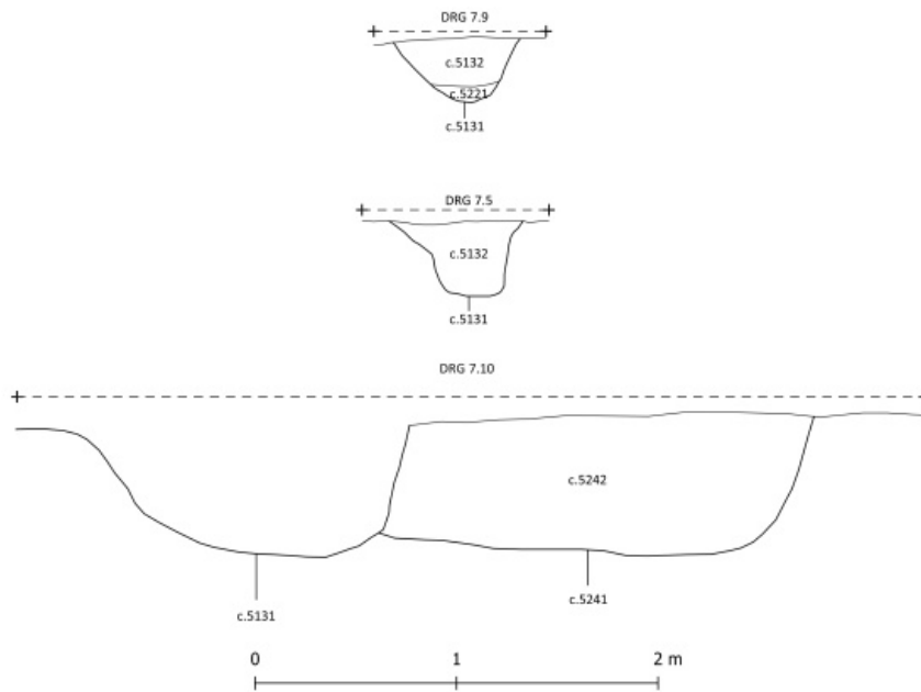
Section of C5131
