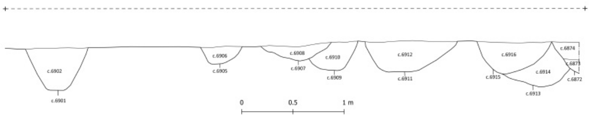
Section through pits and postholes in inner enclosure
