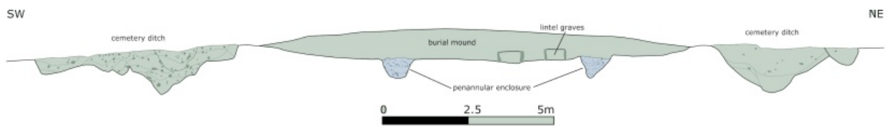
Section through western cemetery
