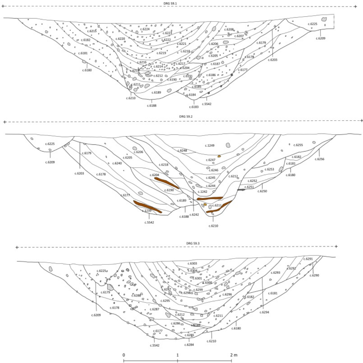
Sections of C5542
